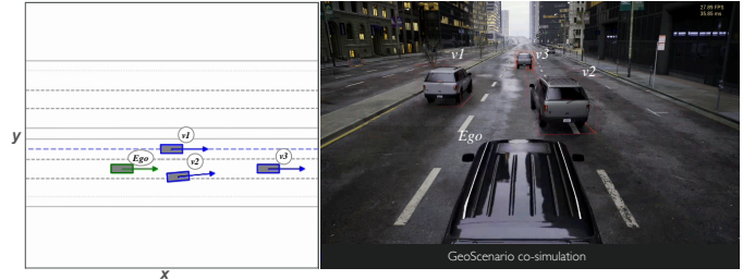
Fig. 1. A challenging interaction between ego and human-operated vehicles based on a pre-crash scenario from NHTSA [2] and using our SDV model in simulation: (left) in the map frame, the SDV Model as v_2 performs the cut-in maneuver targeting ego, and (right) a high-fidelity co-simulator renders the scene.
